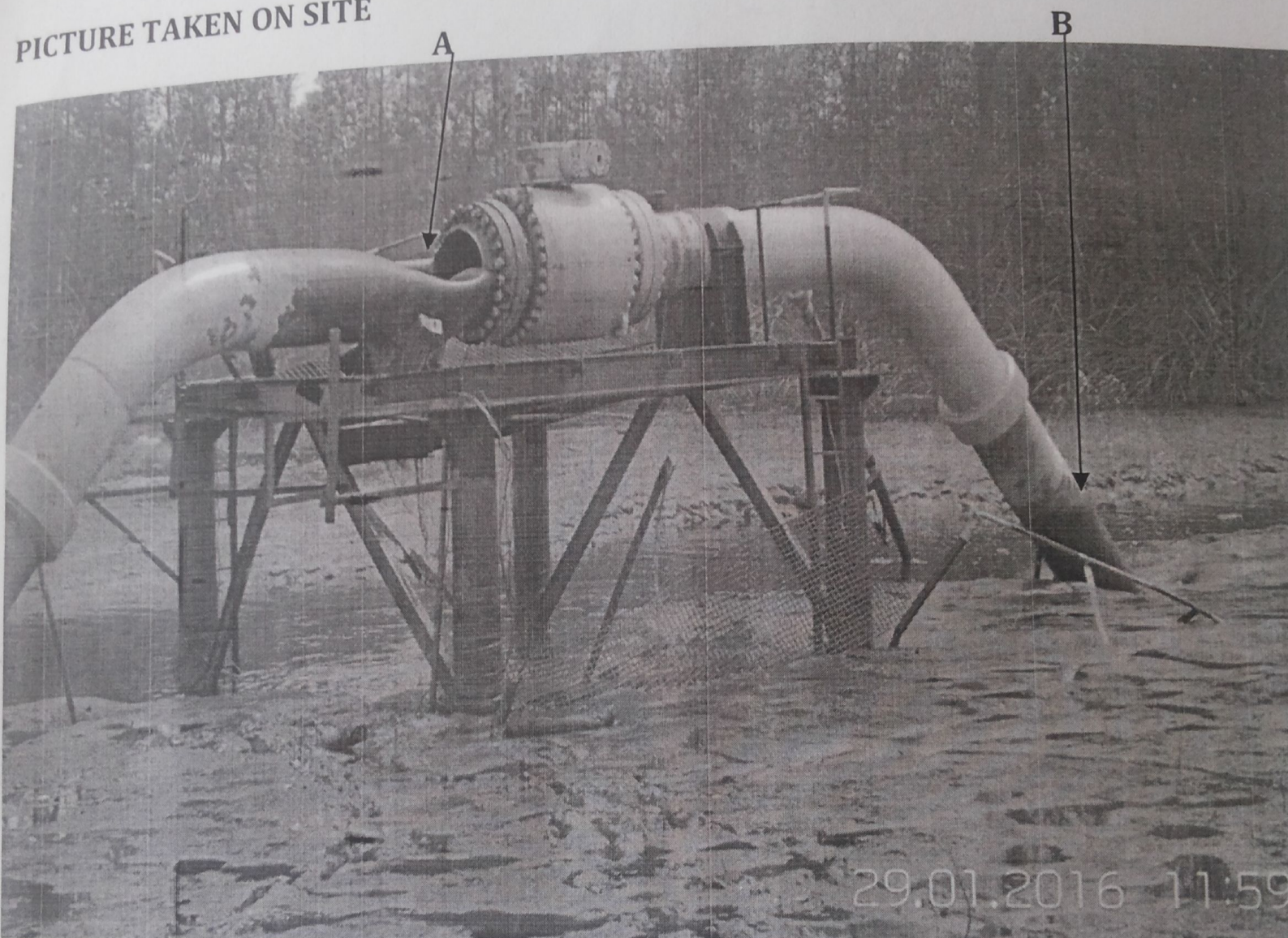
FIG 1: Leak points indicated with black arrow (A is the primary blast point while B is secondary)
